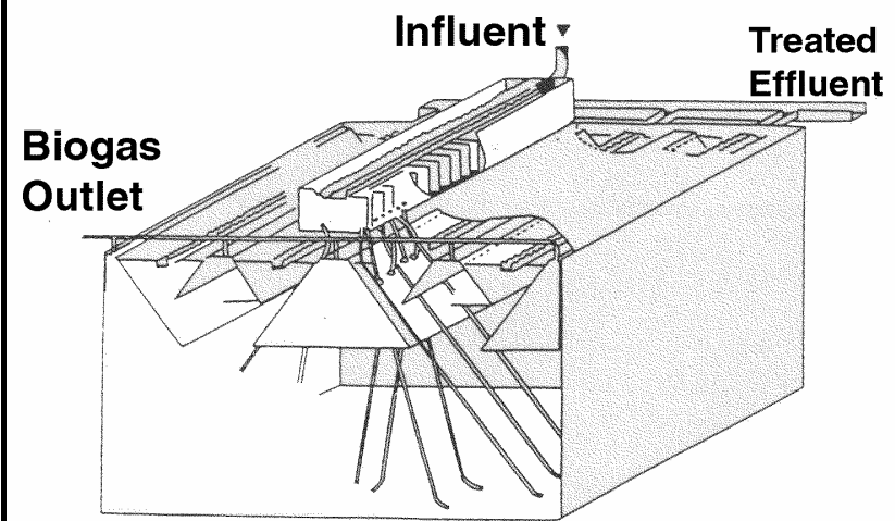
Figure 8.5 Typical UASB Construction
