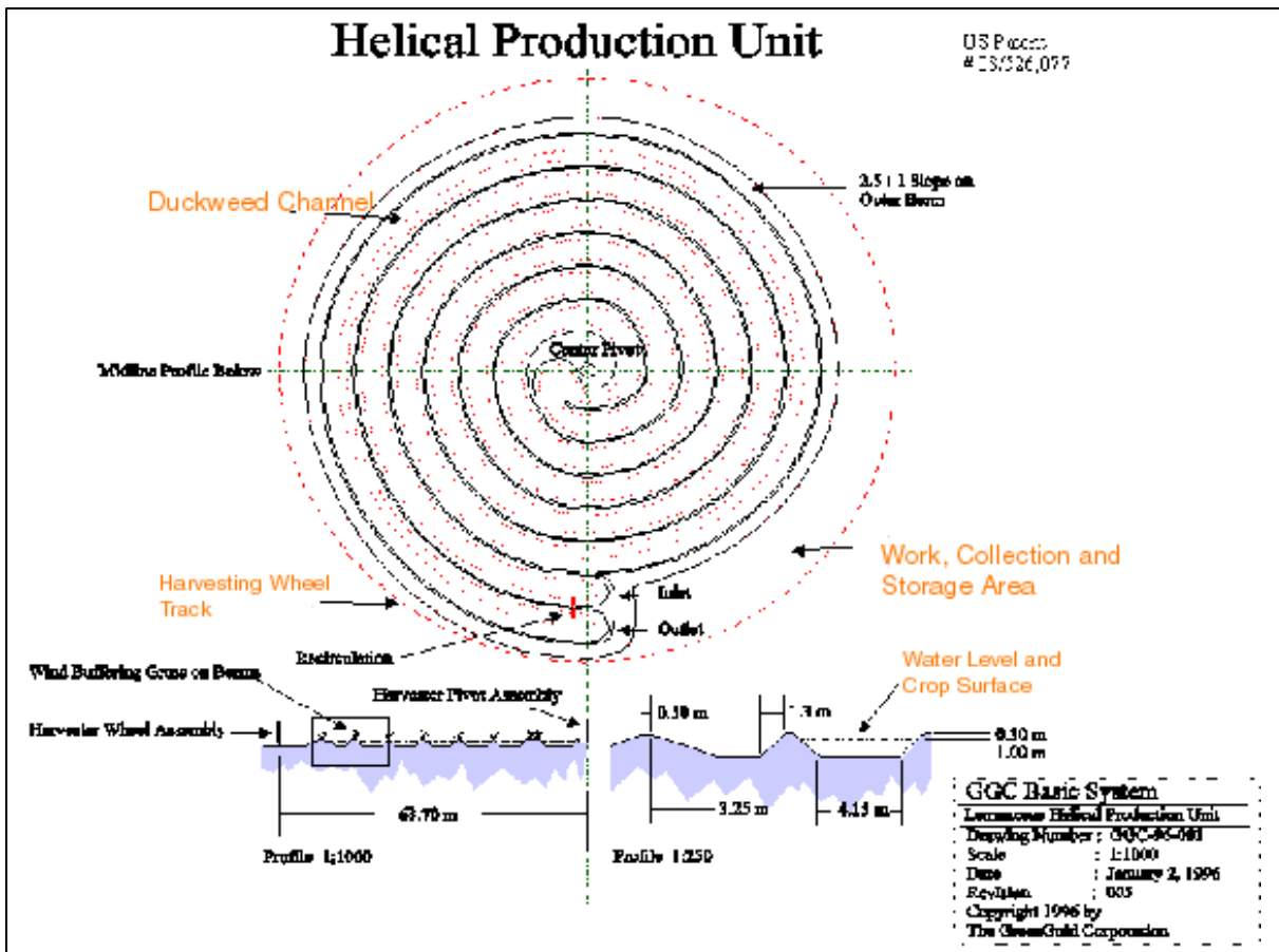
Figure 9.5 GreenGold Duckweed Production Pond Design
