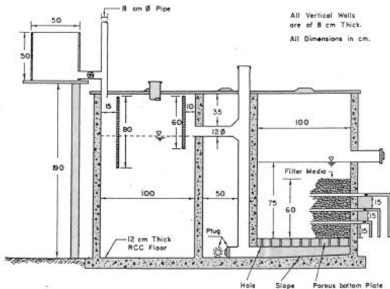
Figure 8.4 Upflow Anaerobic Filter
